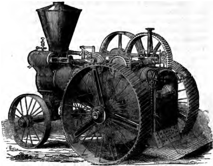
FIG. 117.—The Threshers' Road-Engine, 1878.
